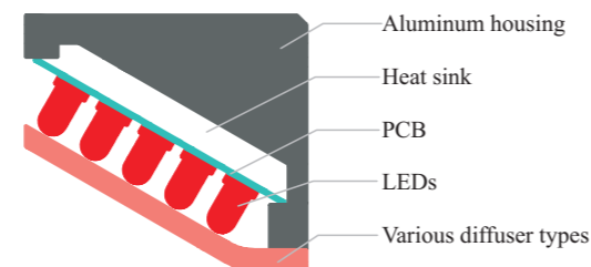
Section Structure Drawing
