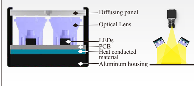
RGB Bar Light Structure Display and Working Way
