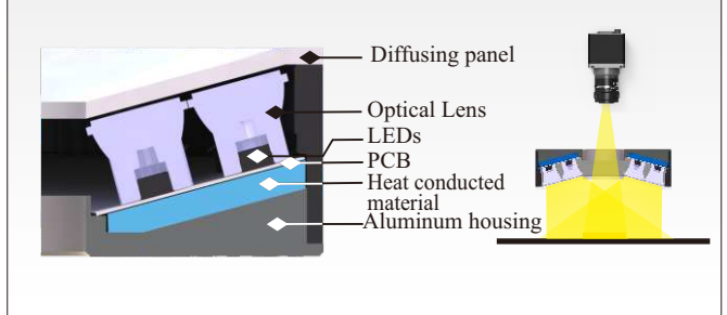
RGB Ring Light Structure Display and Working Way
