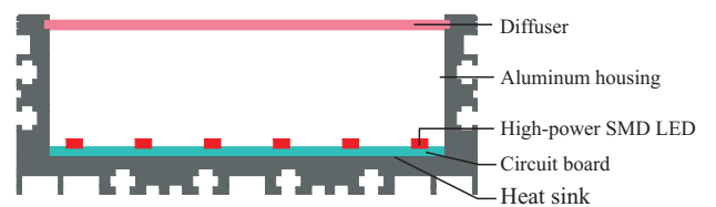
Section Structure Drawing
